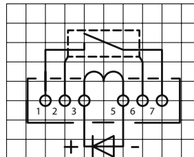
with Diode
